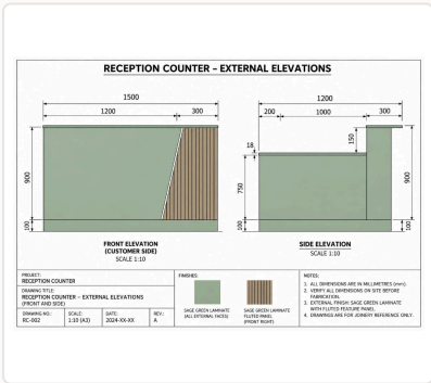
DWG RC-002 (1:10)
