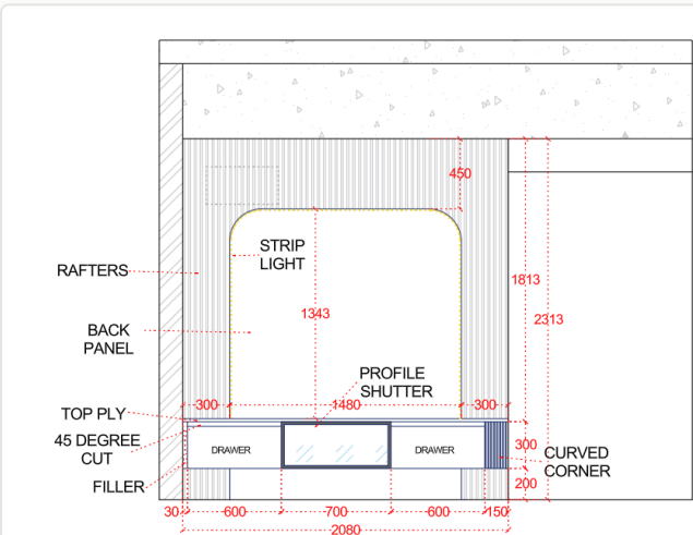
AutoCAD 2D: Living TV Unit Detail (DWG-01, 1:20)
