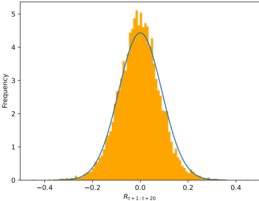
Superimposed R_{t+1:t+20} onto N(0, K\sigma_{t+1}^2)
