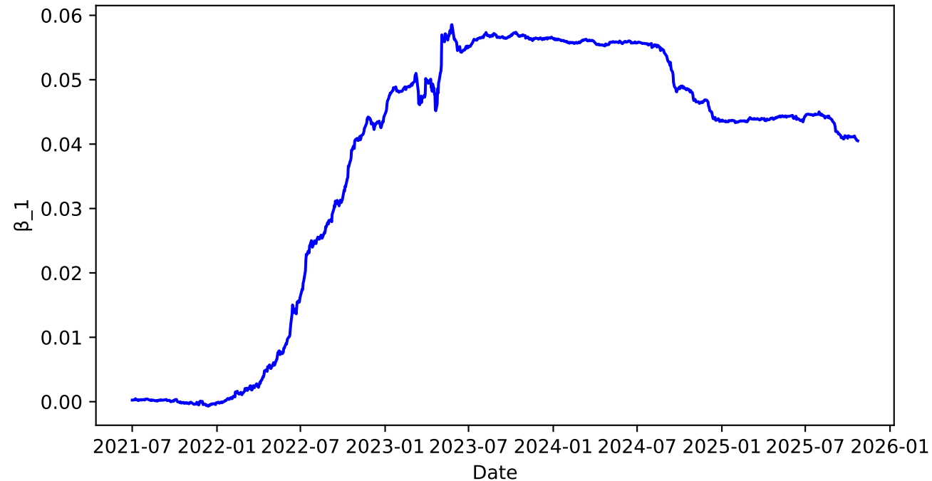
Time Series of \beta_1
