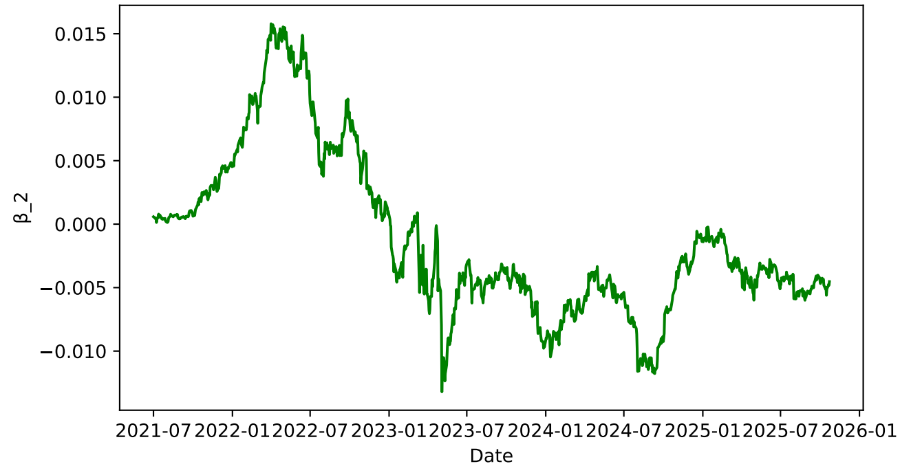
Time Series of \beta_2
