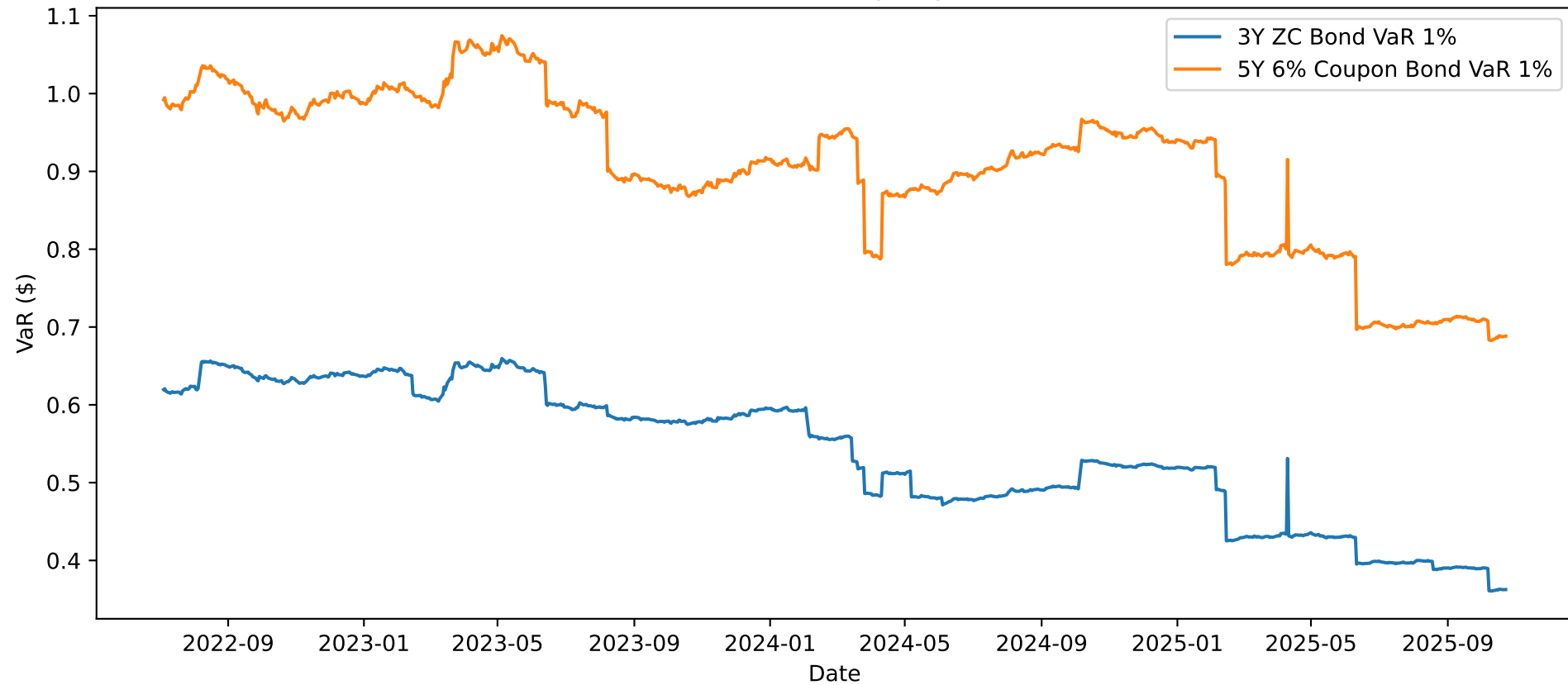
Historical Simulation 1% VaR using Polynomial Term Structure
