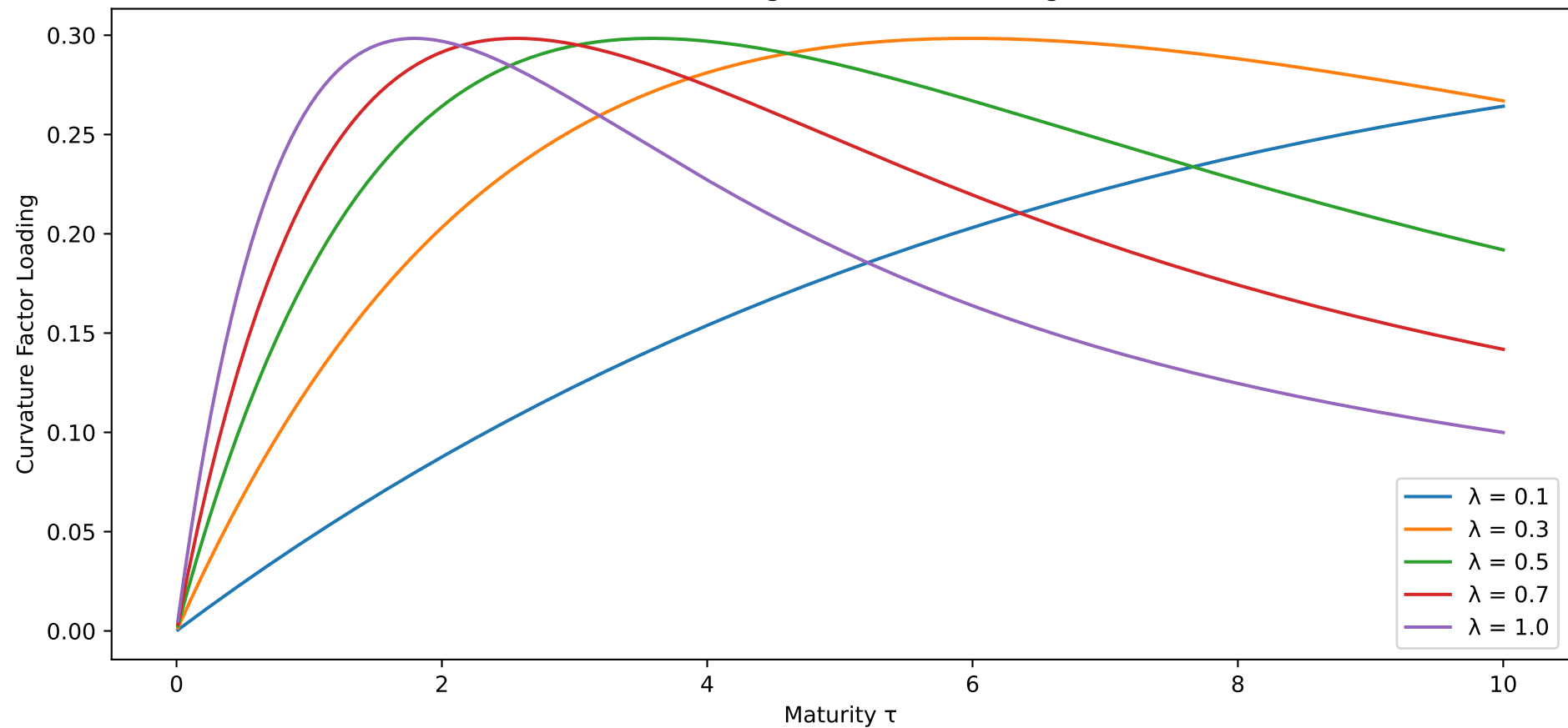
Nelson-Siegel Curvature Loading
