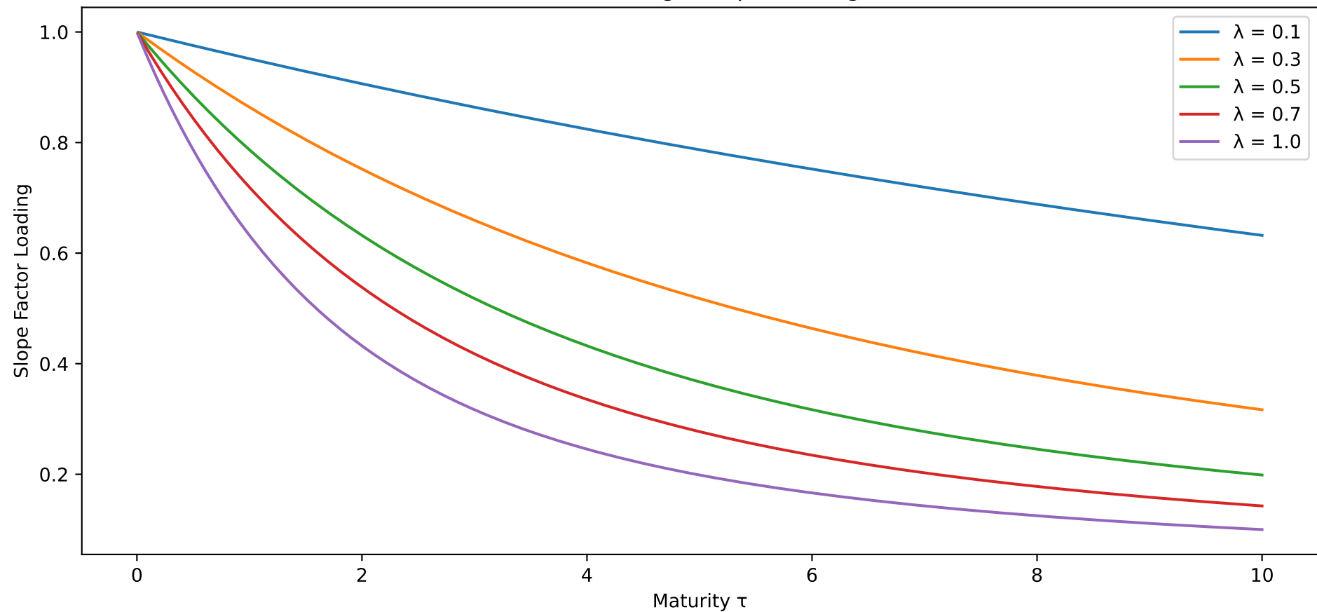
Nelson-Siegel Slope Loading
