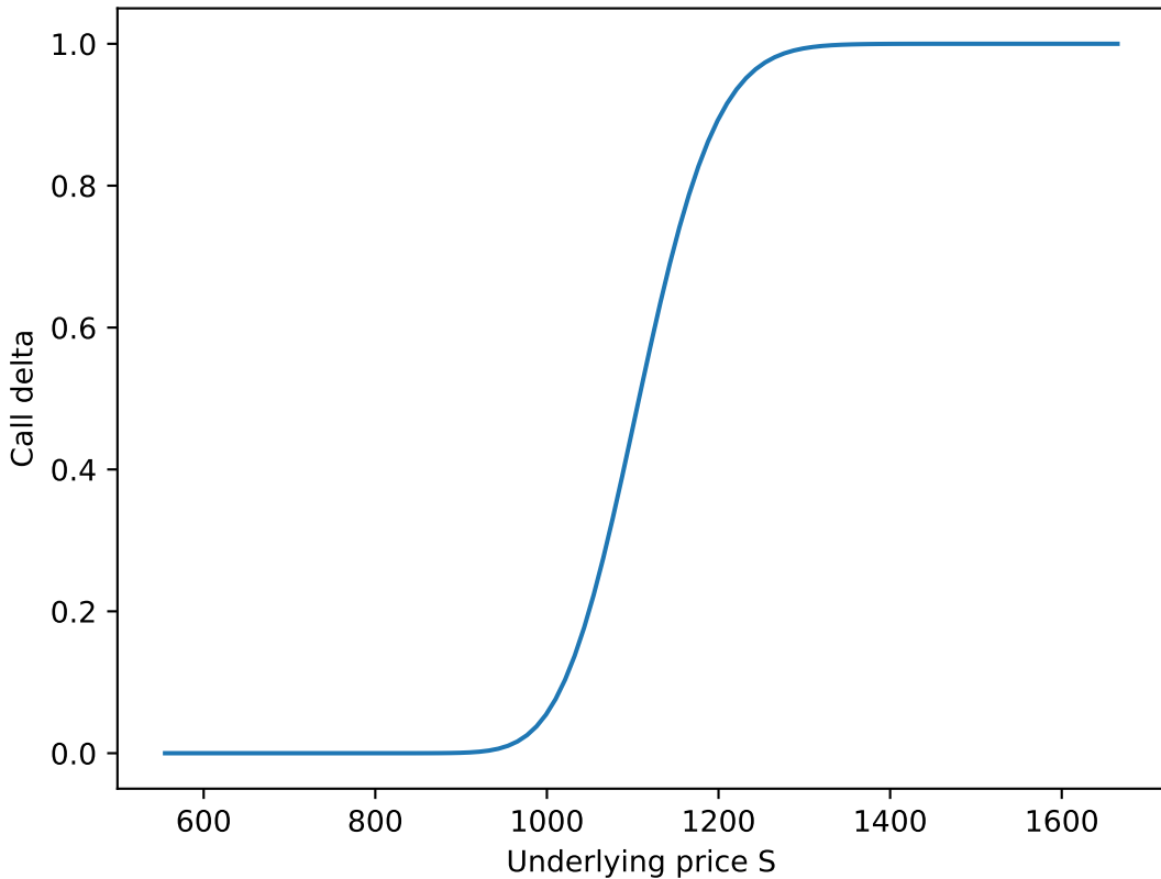
Black-Scholes call delta as a function of S
