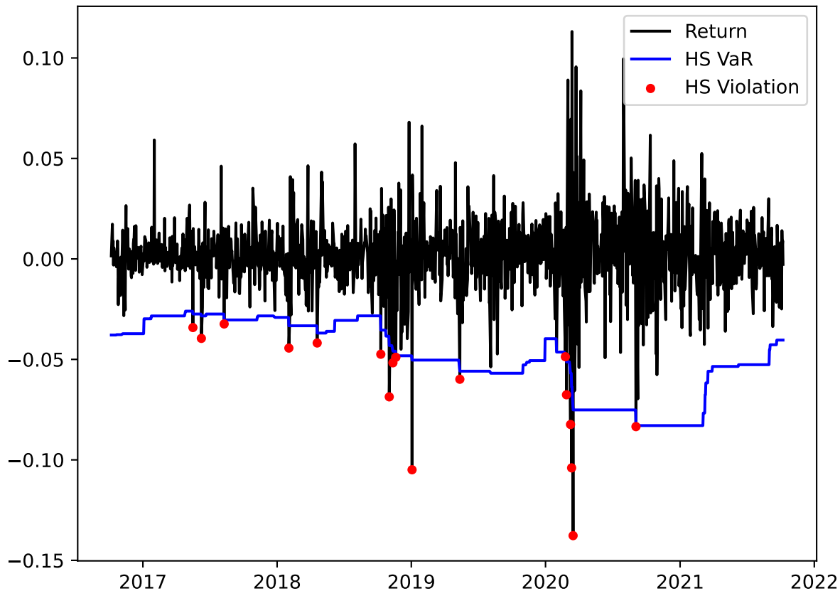
Apple — HS VaR Backtest
