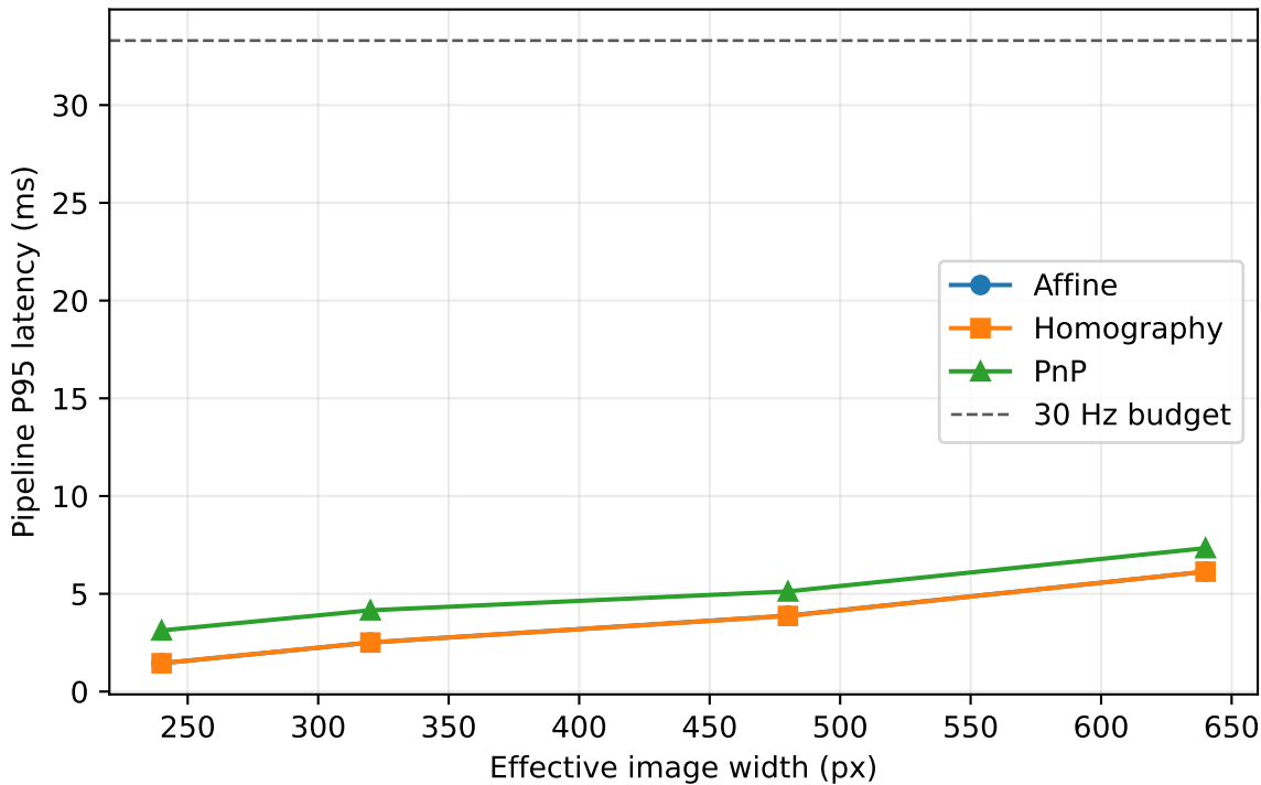
E5 detection + mapping latency — ihawk2
