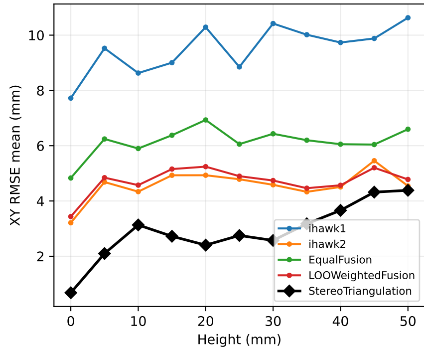
E6 independent PnP estimates versus true two-view geometry XY localization
