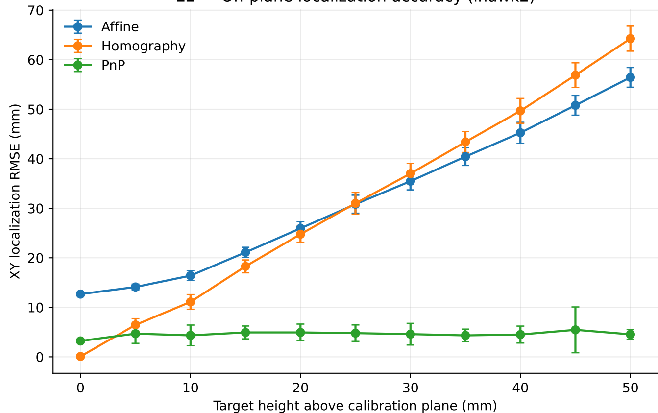
E2 — Off-plane localization accuracy (ihawk2)
