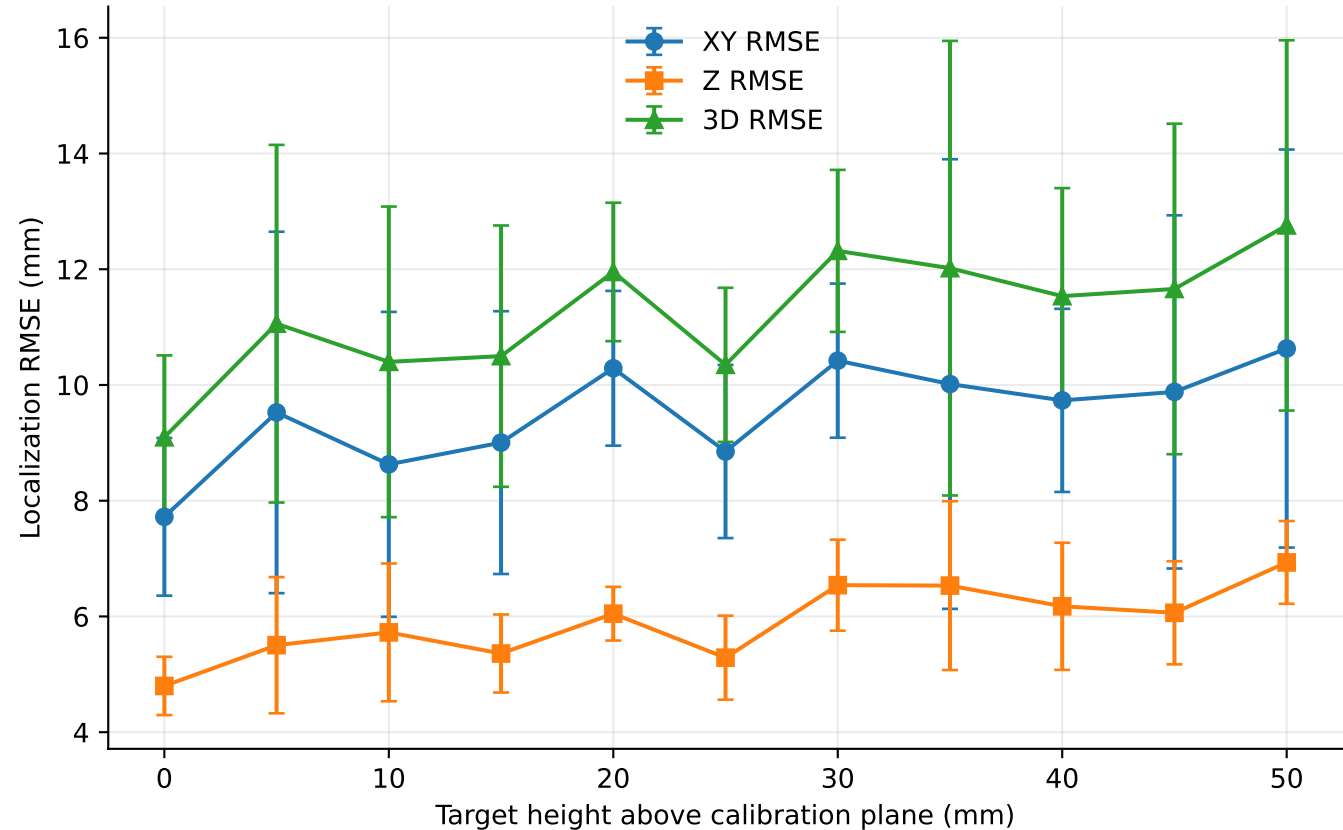
E2 — PnP 3D localization performance (ihawk1)
