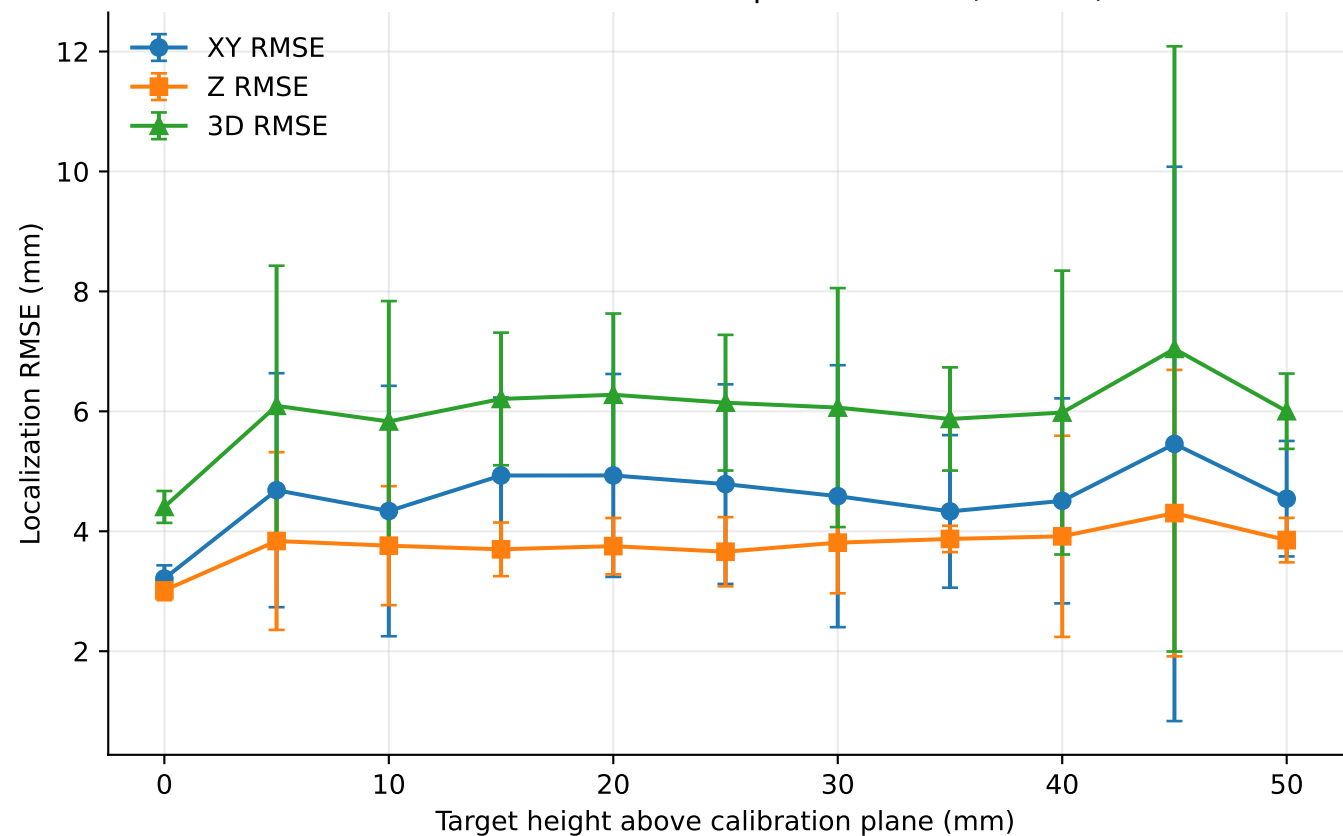
E2 — PnP 3D localization performance (ihawk2)
