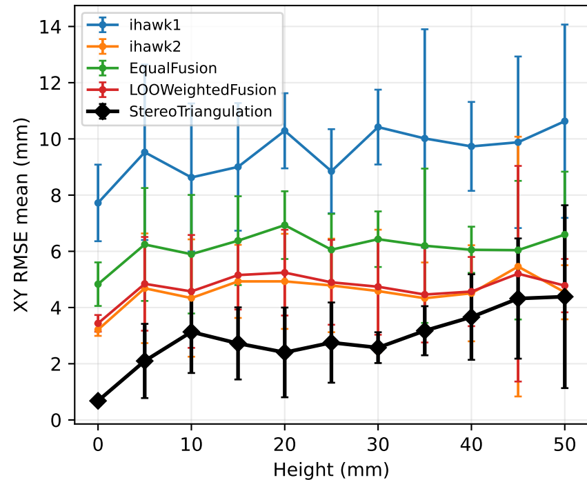
E6 independent PnP estimates, estimate fusion, and two-view geometry XY localization
