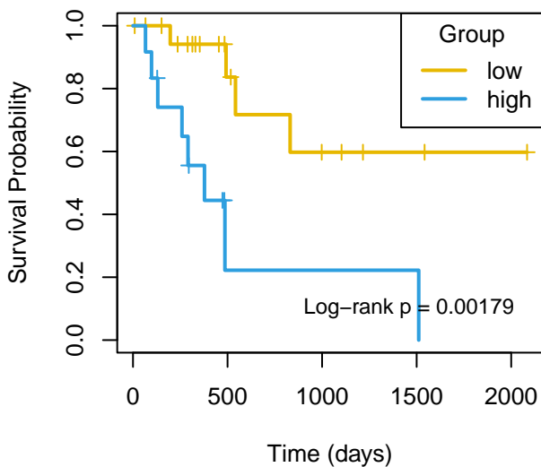
DFI mir-193b
