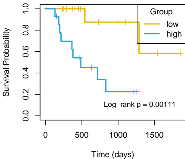
DFI mir-584
