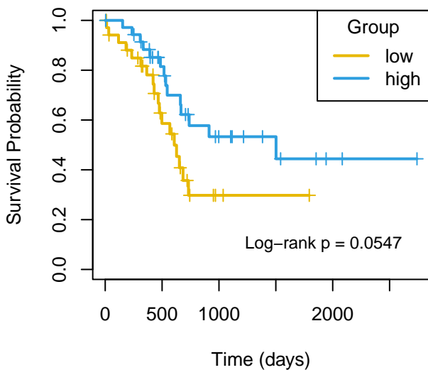
OS mir-652
