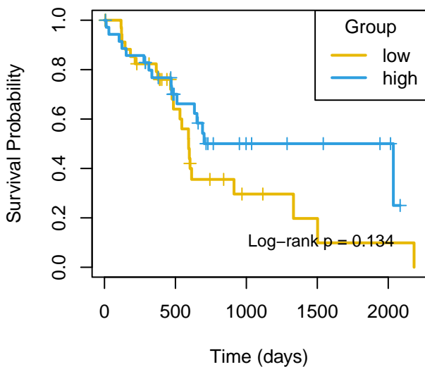
OS mir-30b
