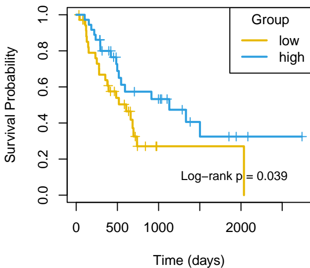
OS mir-129-2
