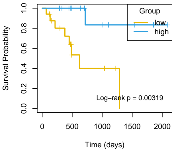
DFI mir-5683
