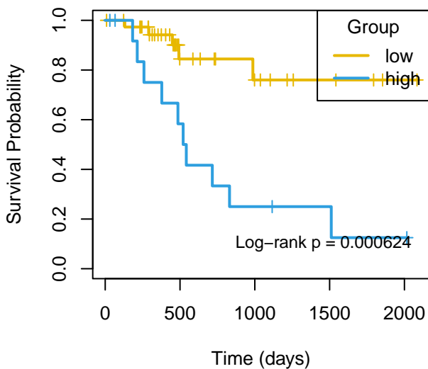
DFI mir-5580
