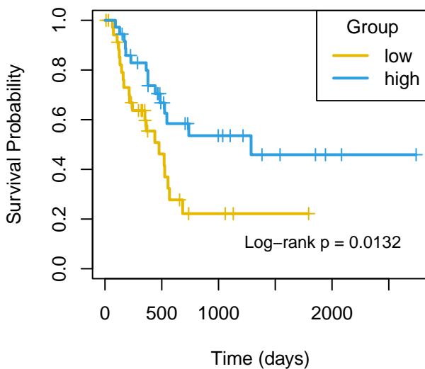
PFI mir-324
