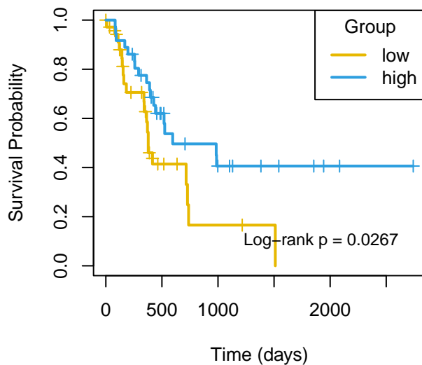
PFI mir-1224
