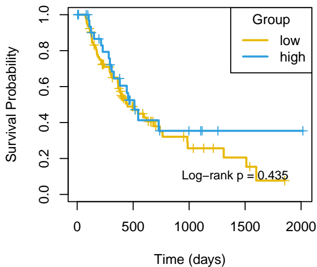
PFI mir-320c-2
