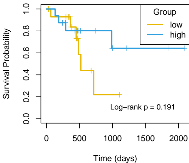
DFI mir-186
