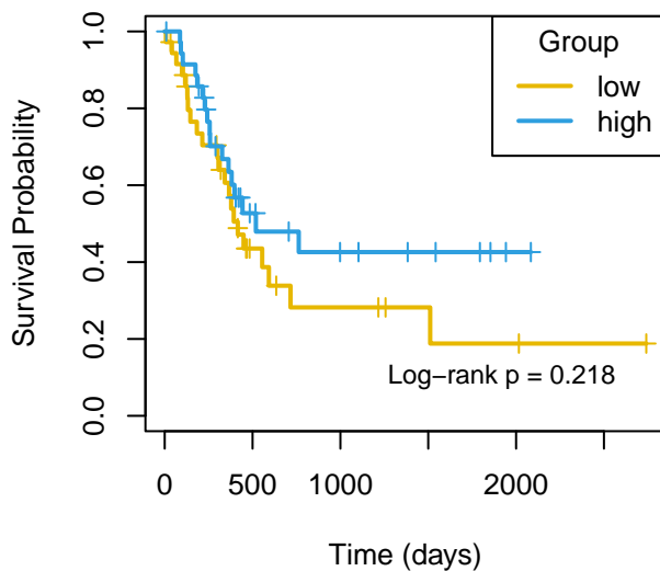
PFI mir-889
