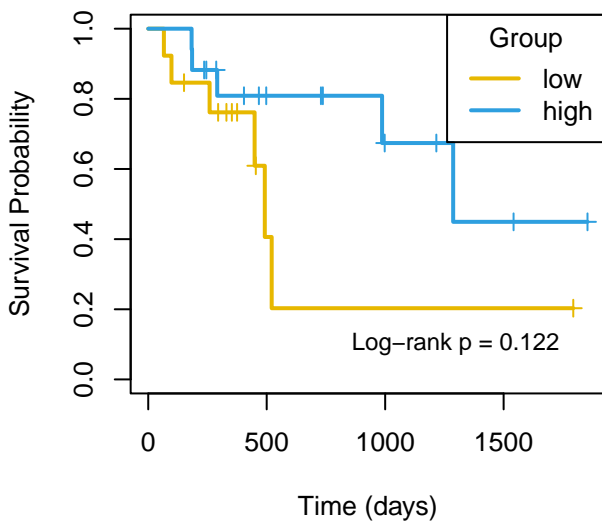
DFI mir-103a-1
