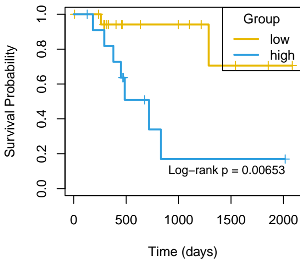
DFI mir-203a
