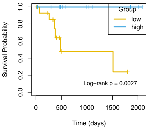
DFI mir-29c
