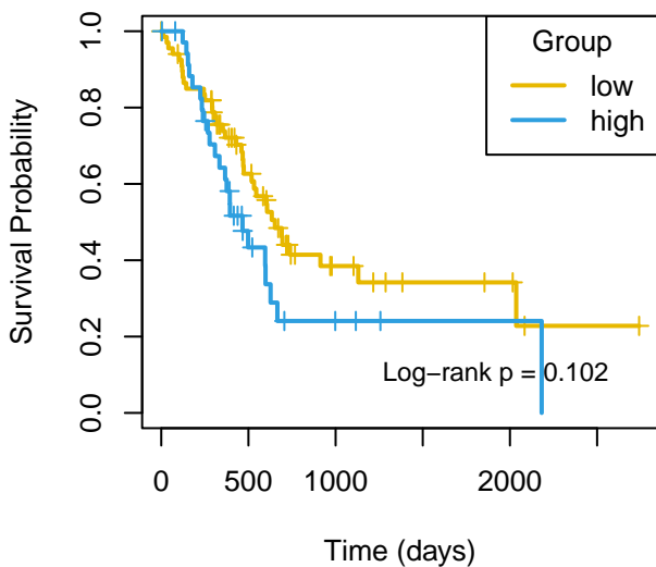
OS mir-1294
