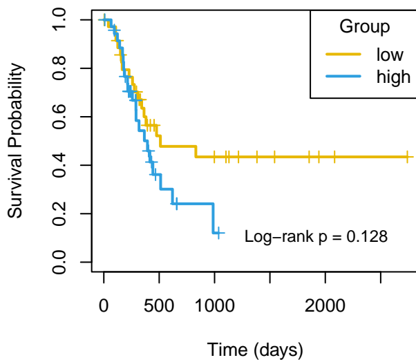
PFI mir-146b
