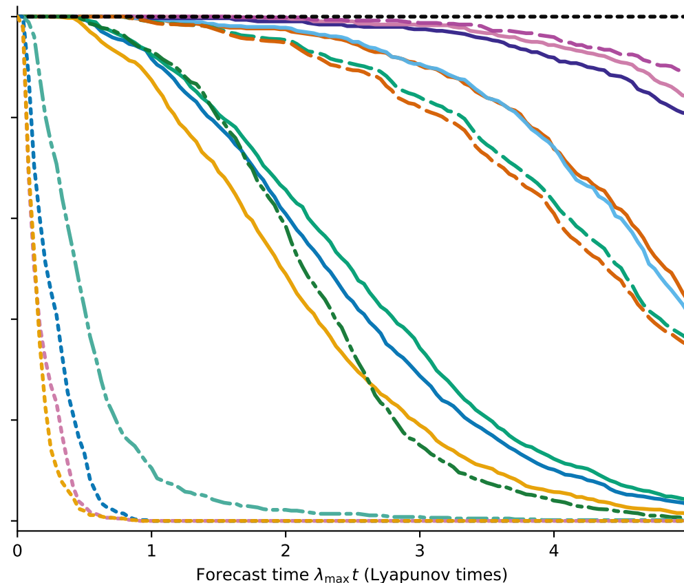
Benchmark training noise 1%
