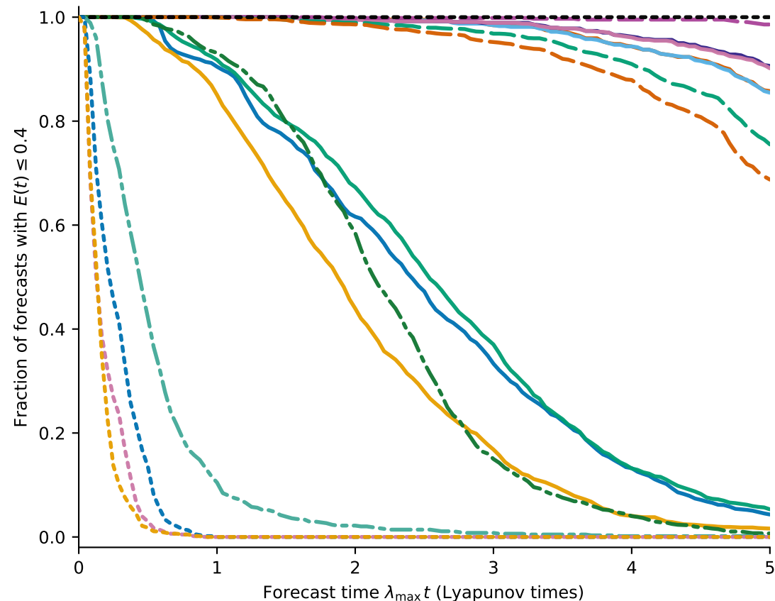
Benchmark training noise 0.1%
