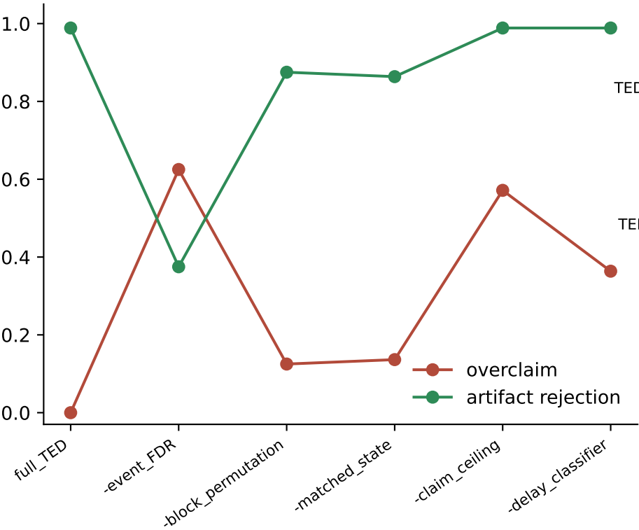
C Ablation exposes functional safeguards
