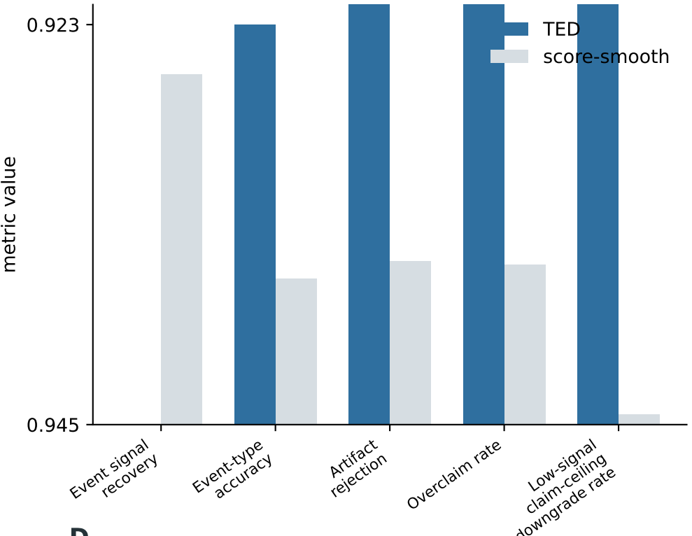
D Variant selection rejects claim inflation
