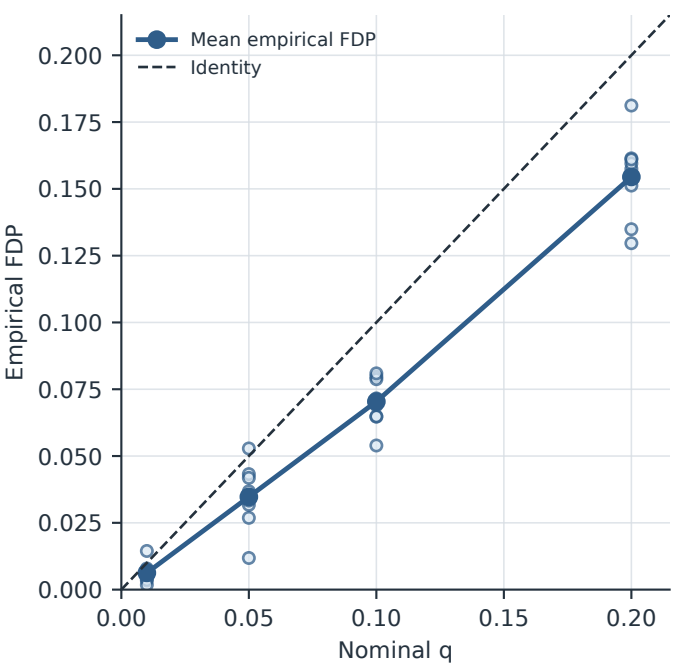
D. Event-FDR calibration
