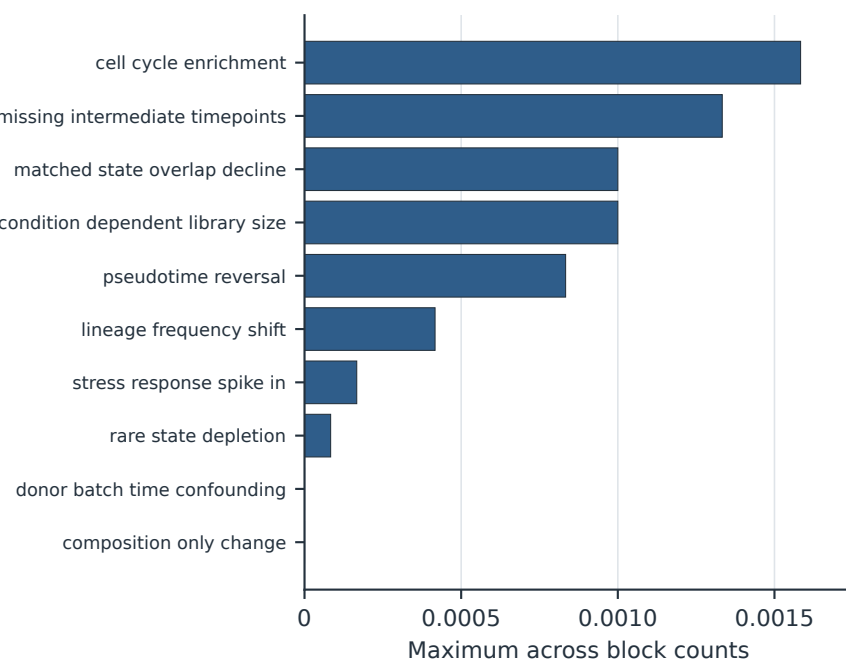
F. Confounded-null false escalation
