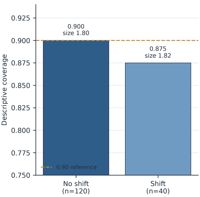
E. Ambiguity-aware set coverage
