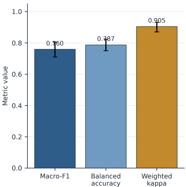
B. Classification and legacy-tier agreement
