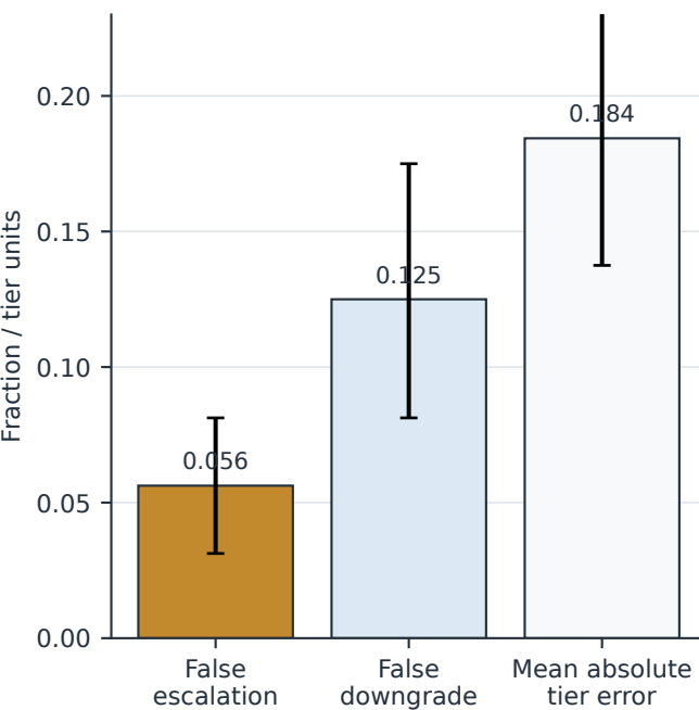
C. Legacy evidence-tier errors
