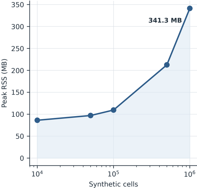
E. Peak resident memory
