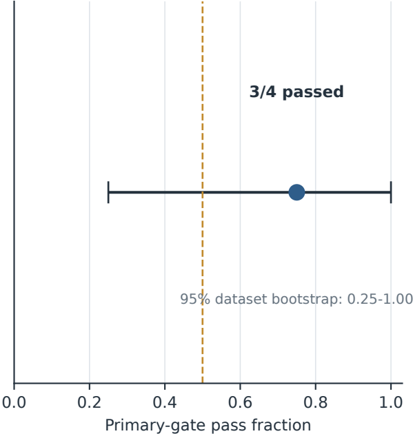
B. Four-dataset frozen-gate audit
