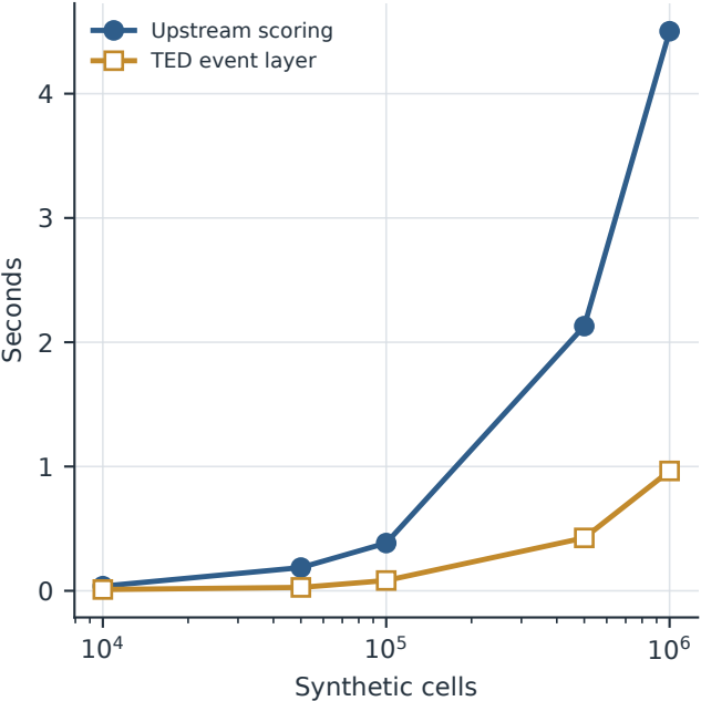
D. Scaling time by component
