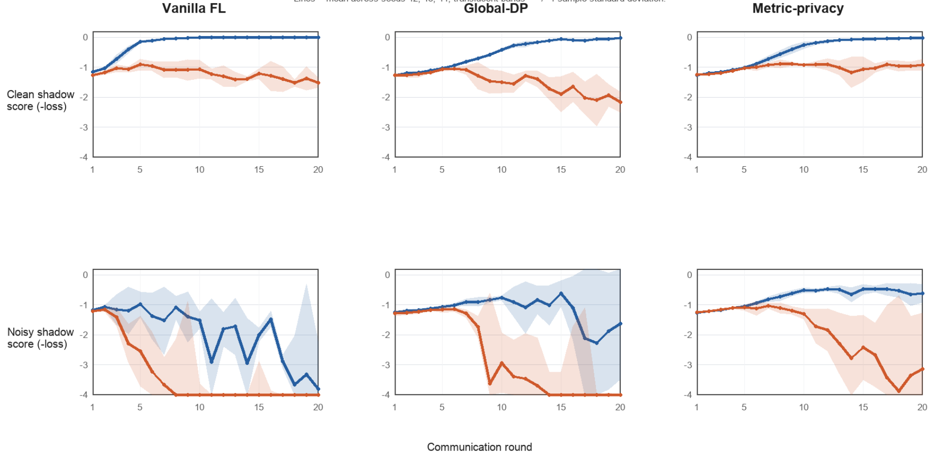
Figure 1: CIA score trajectories. Each panel uses raw scores s_r = -\mathcal{L}(W^{(r)}, D_x) and the shared y-axis range [-4, 0.2] .
