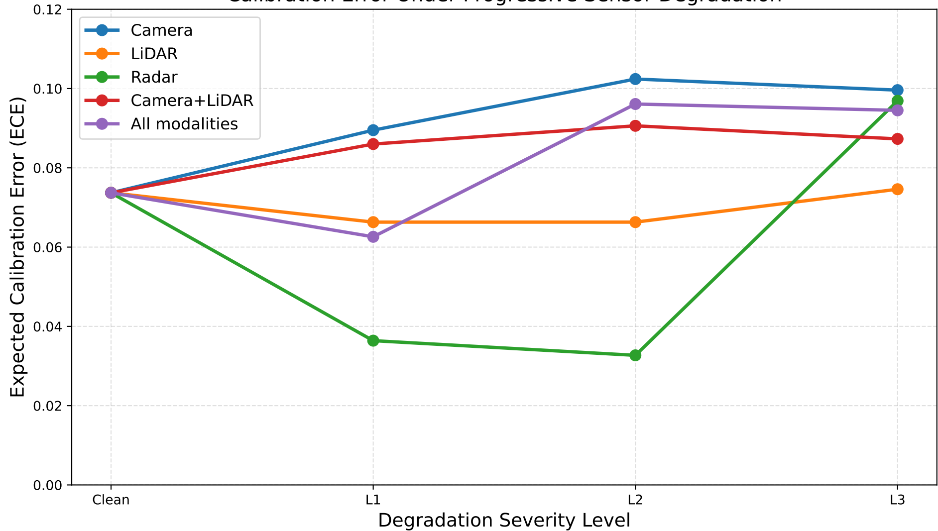
Calibration Error Under Progressive Sensor Degradation
