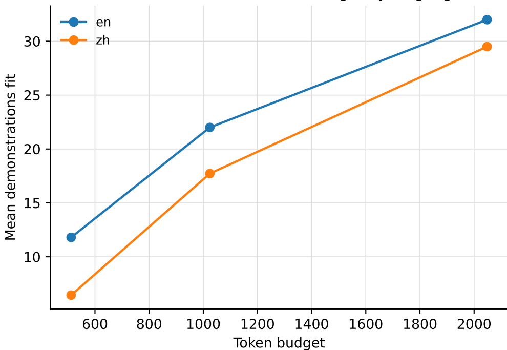
Demonstrations that fit into budget by language
