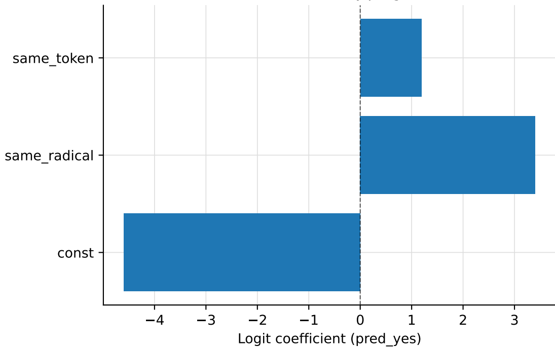
Drivers of similarity judgment
