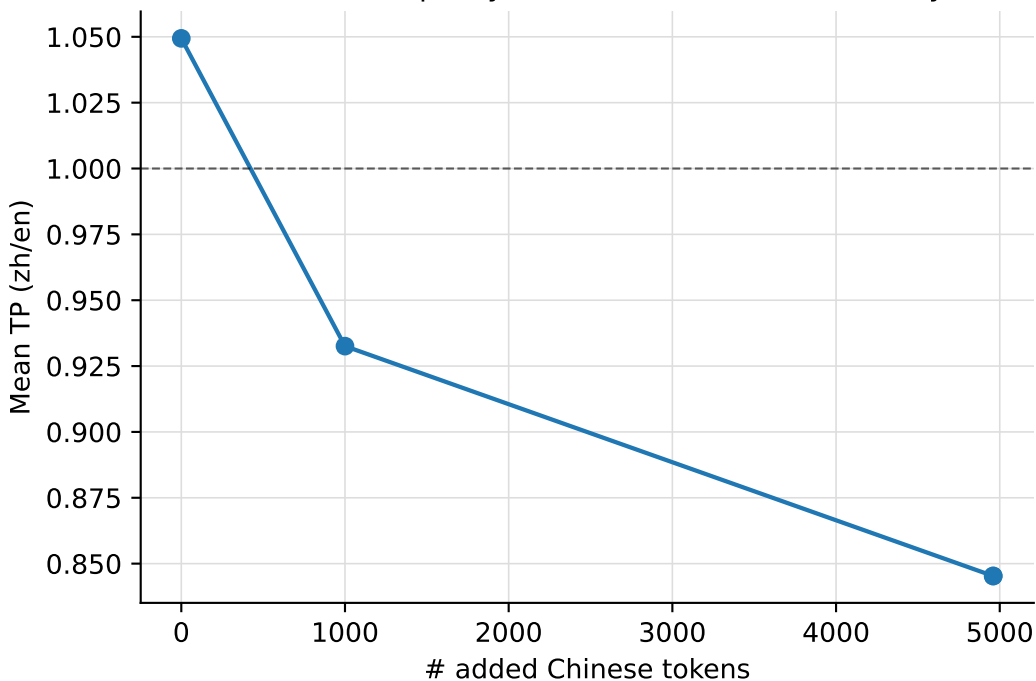
Tokenization parity vs added Chinese vocabulary
