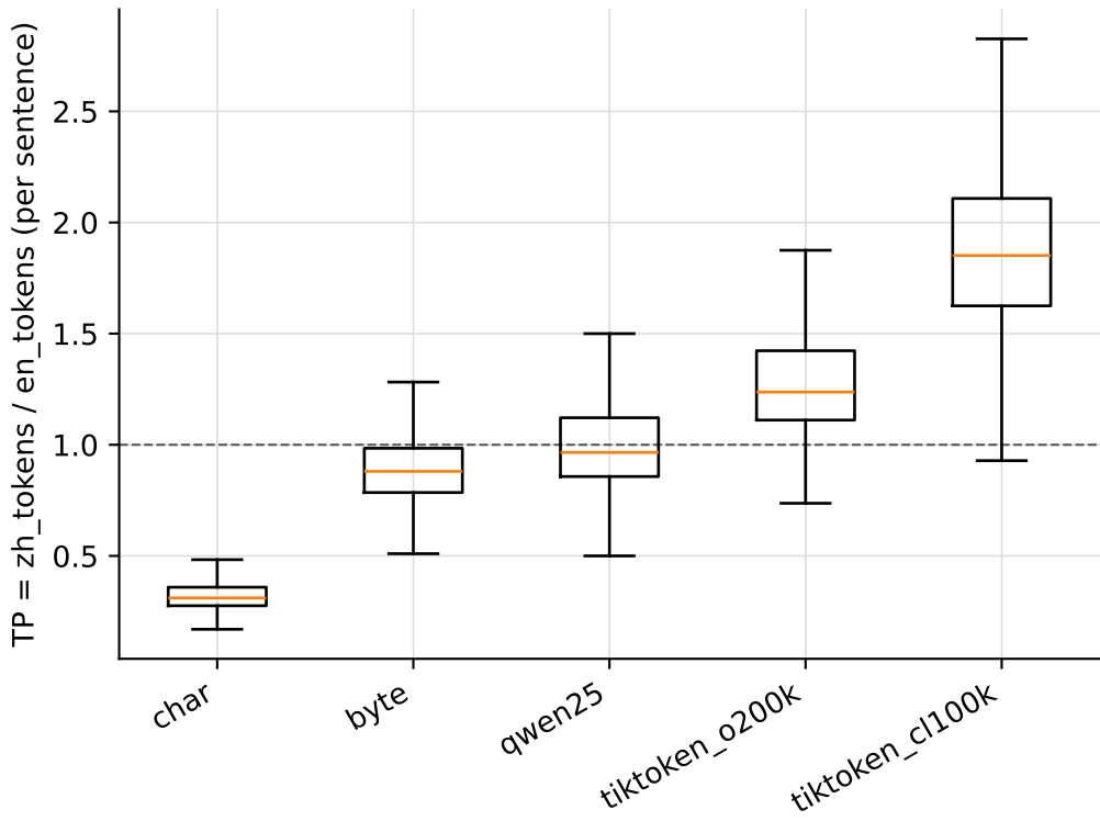
Per-sentence tokenization parity by tokenizer
