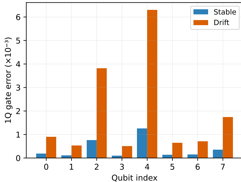
1Q gate error inflation
