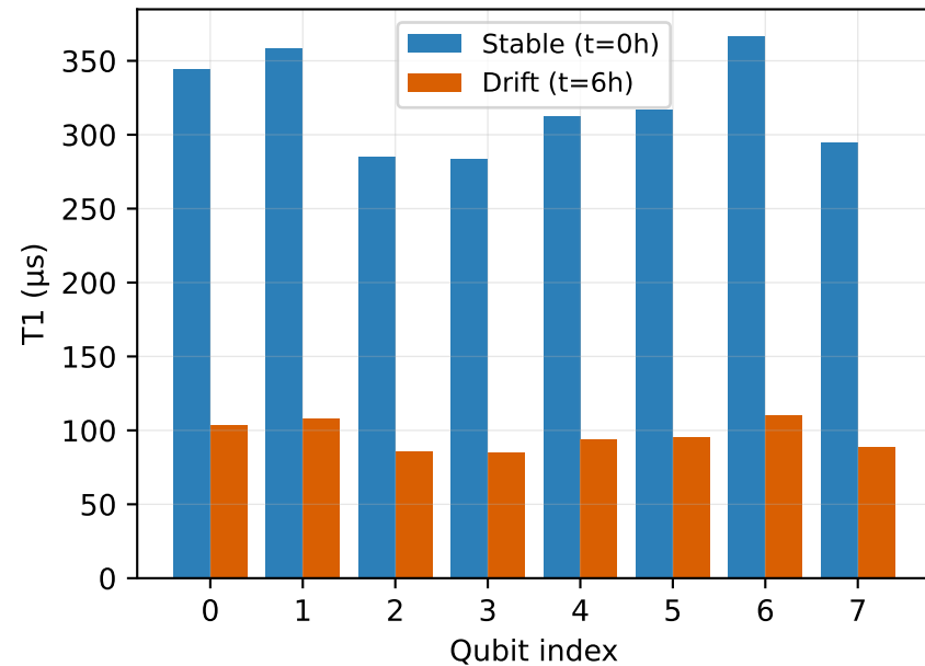
T1 collapse after drift
