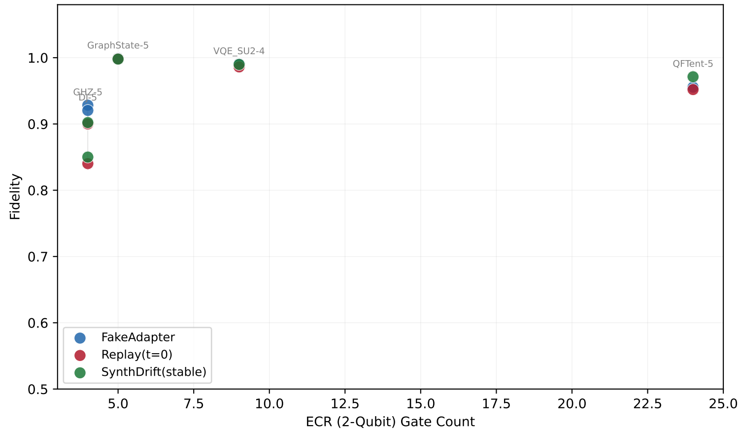
Fidelity vs 2Q Gate Count
