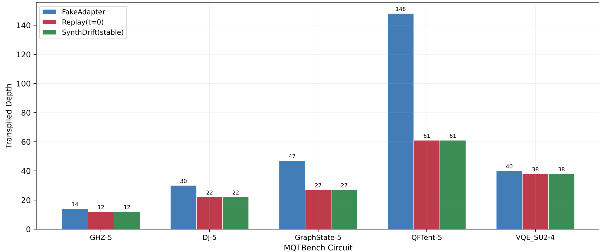
Transpiled Circuit Depth on Each Backend
