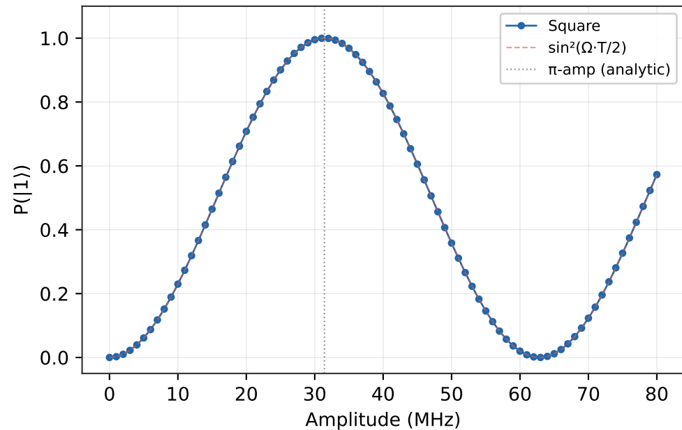
Square Pulse (T=100 ns)
