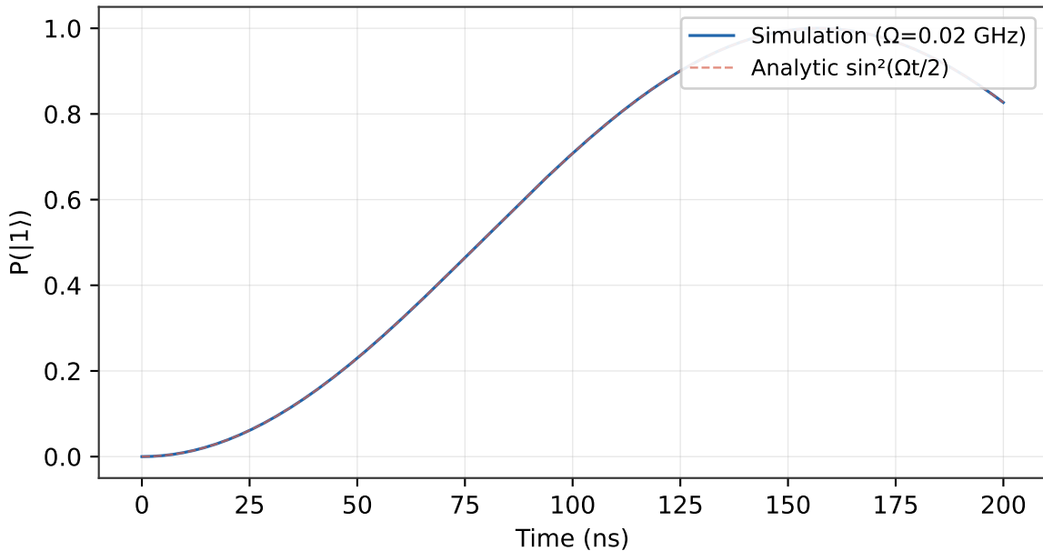
Rabi Oscillation — Time Evolution (Square Pulse)
