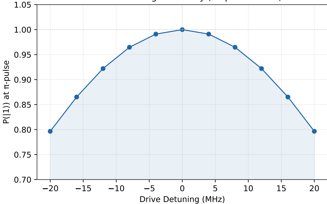
\pi -Pulse Detuning Sensitivity (amp=52.7 MHz)
