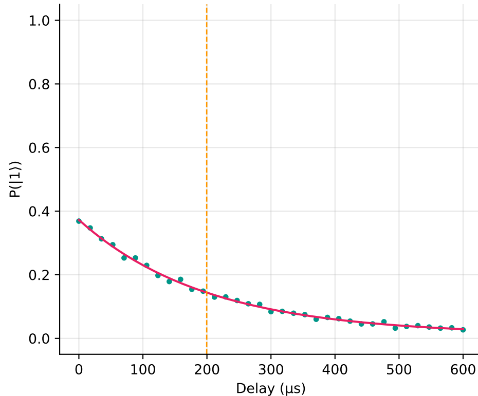
T1=200 \mu s ( R^2=0.996 )
