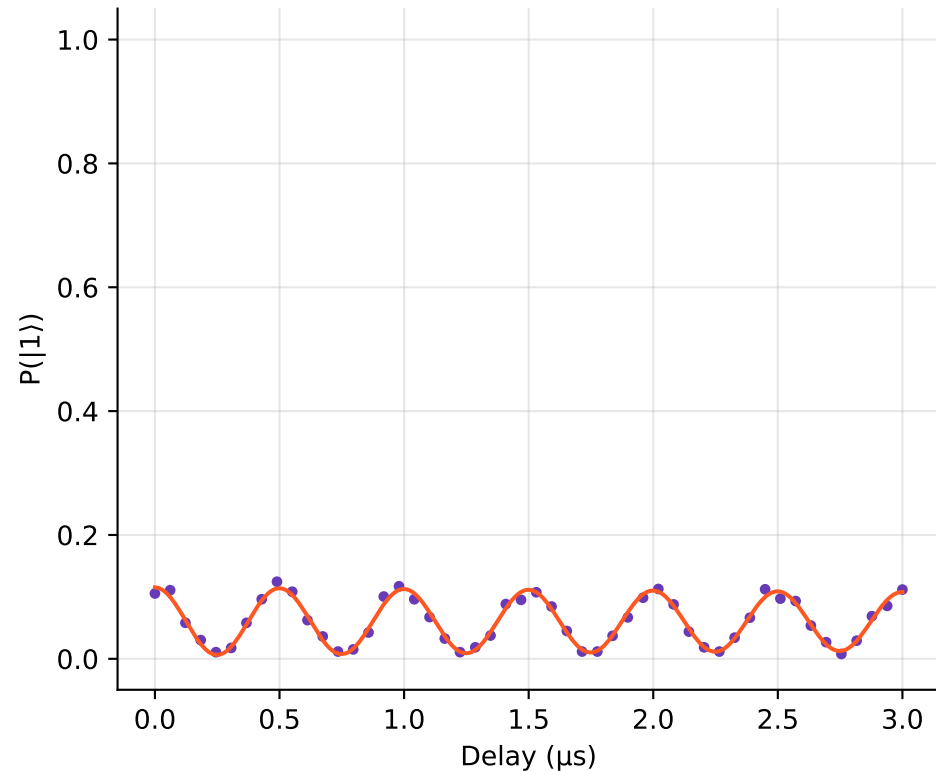
Ramsey T2*=20.4 \mu s ( R^2=0.973 )
