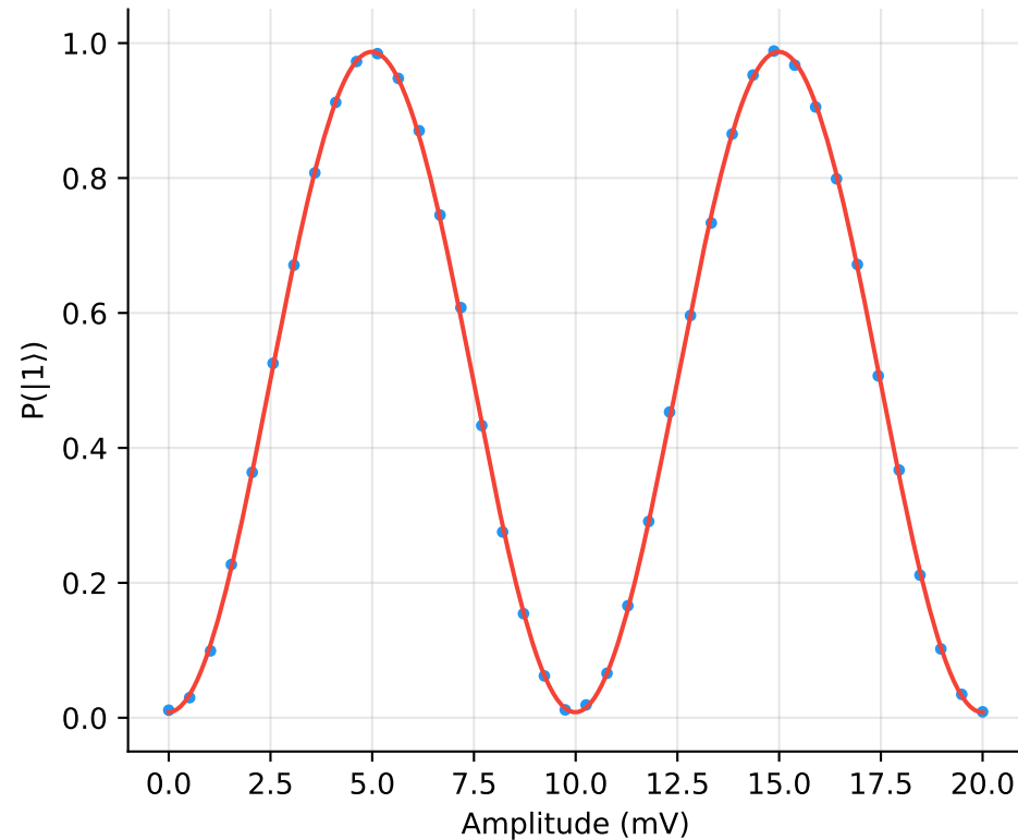
Rabi ( R^2=1.000 )
