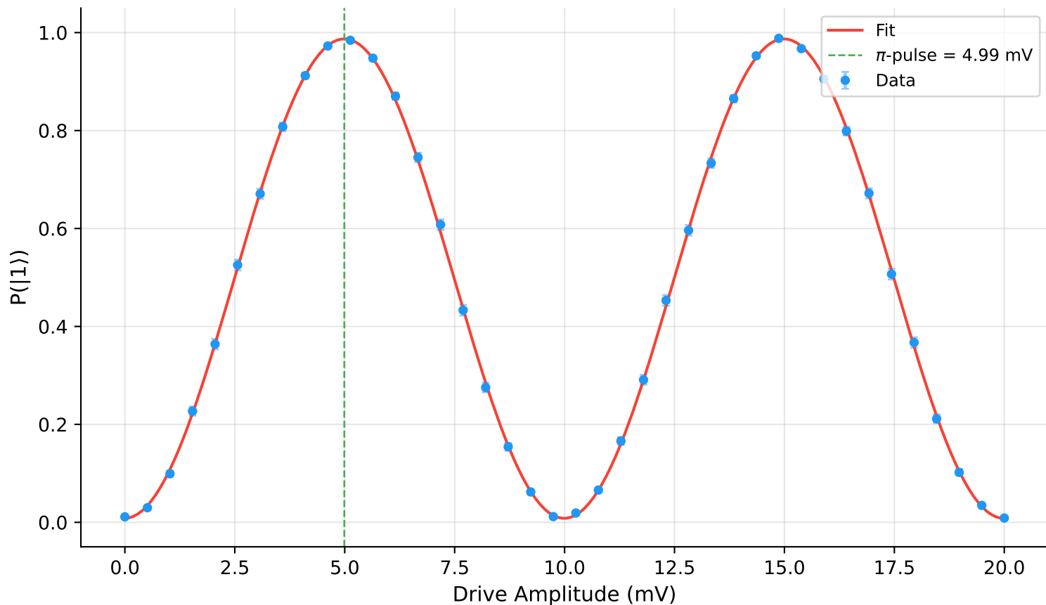
Rabi Oscillation (Q0) — R^2 = 1.000
