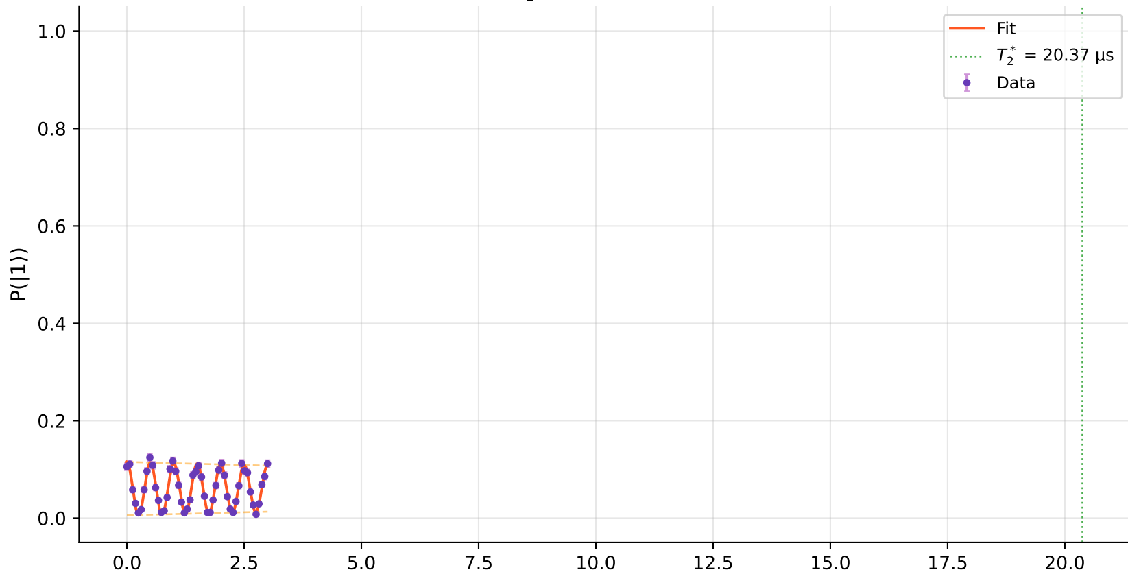
Ramsey Fringes (Q0) — T_2^* = 20.37 \mu\text{s} , \Delta f = 2.00 \text{ MHz} , R^2 = 0.973
