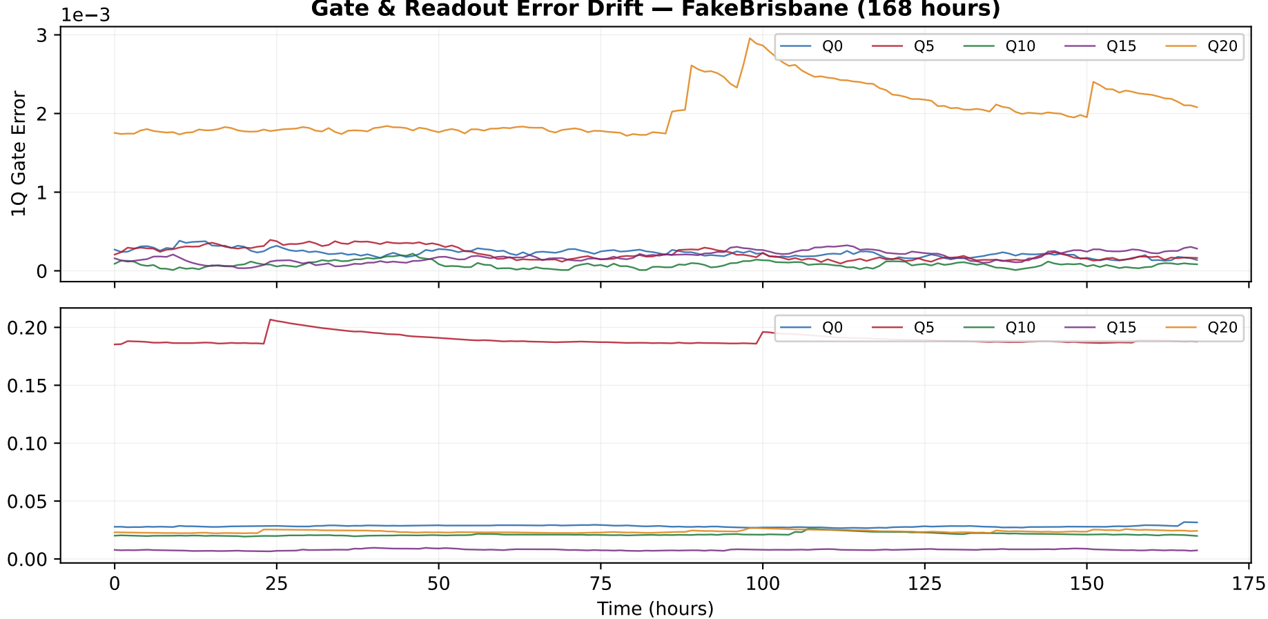
Gate & Readout Error Drift — FakeBrisbane (168 hours)
