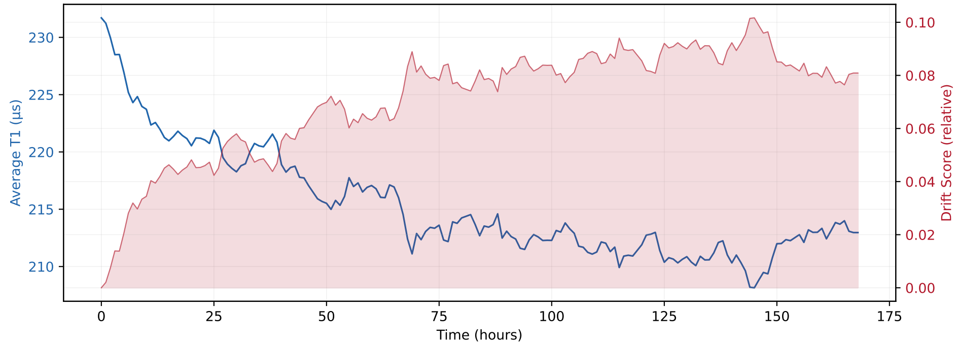
ReplayBackend — Average T1 & Drift Score Over Time
