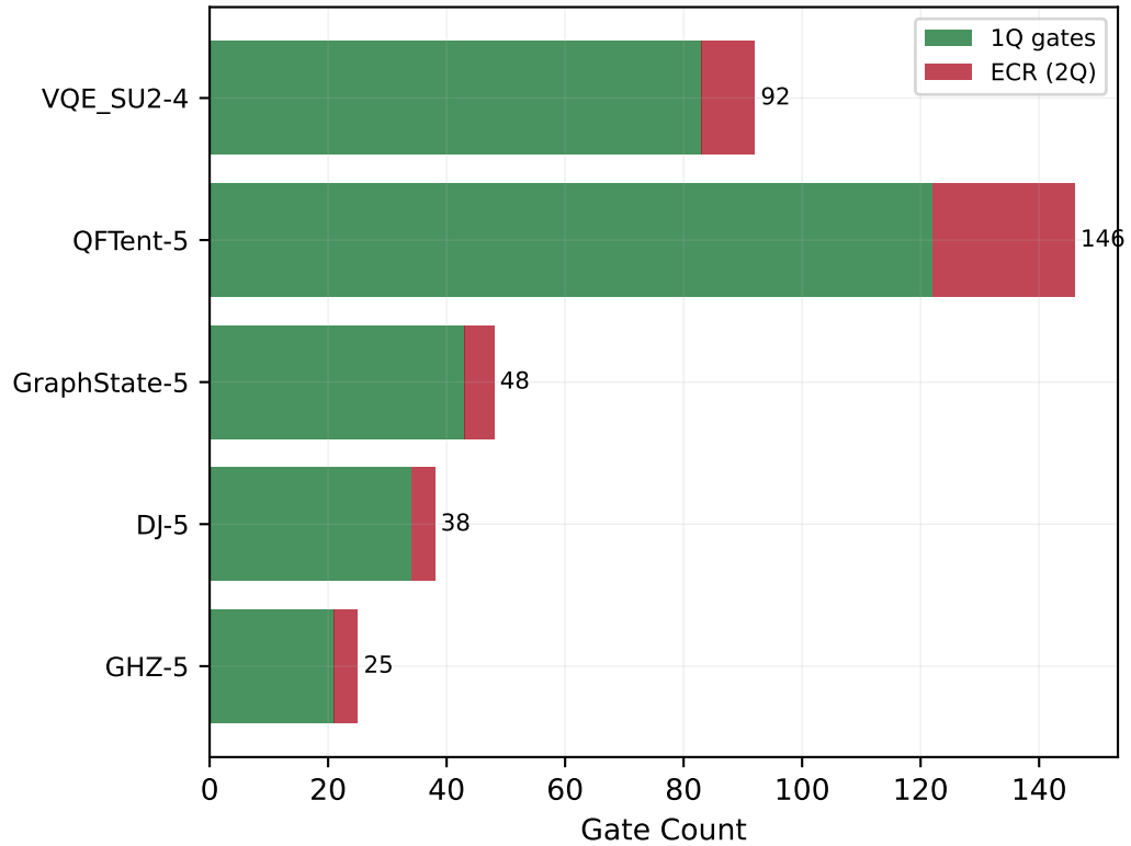
Gate Composition (IBM Eagle)
