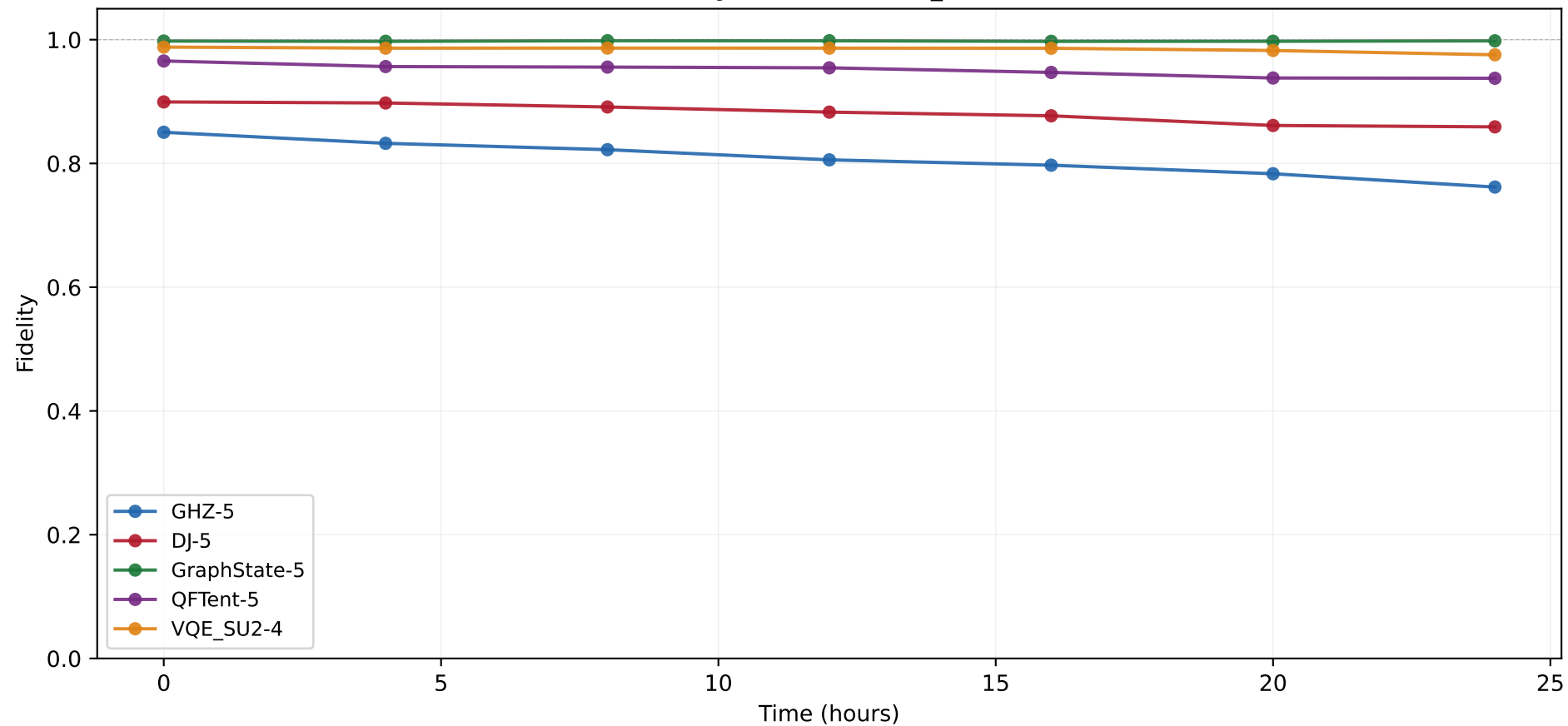
MQTBench Fidelity Under LINEAR_DECAY Drift (24h)
