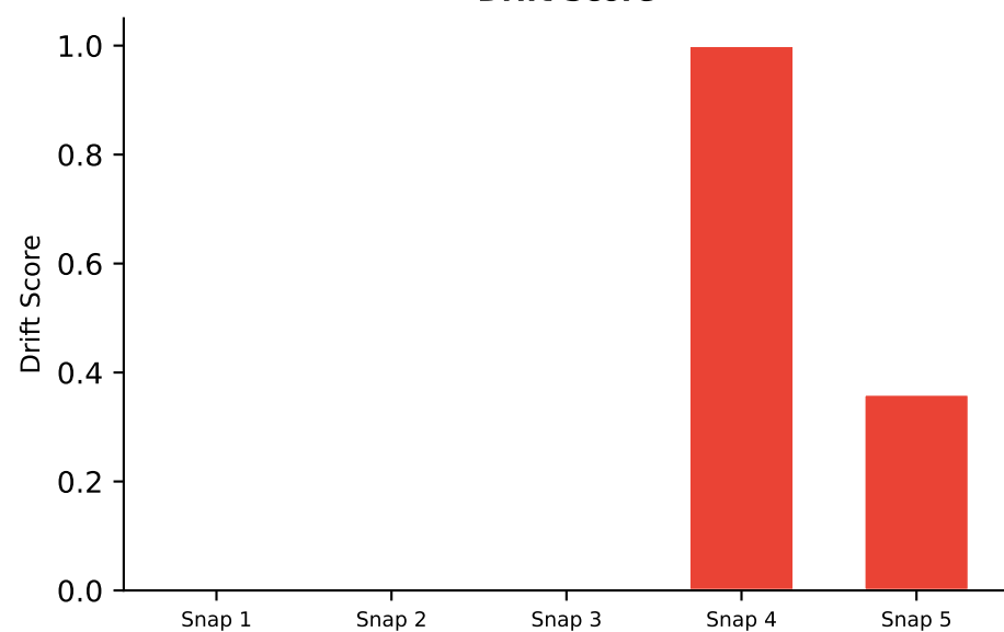
Drift Score
