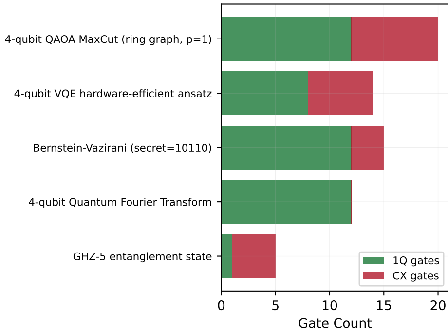
Gate Composition
