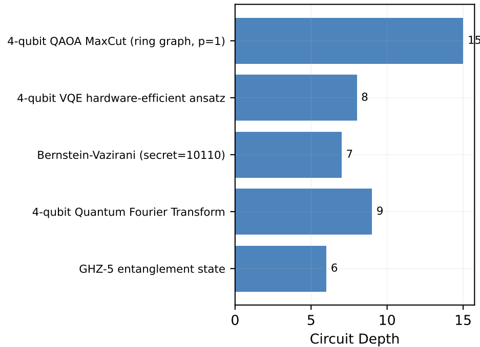
Circuit Depth
