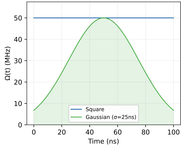
Drive Envelopes
