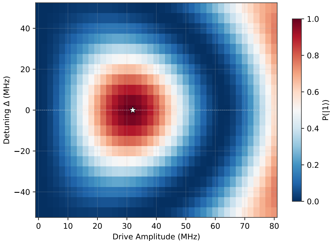
Rabi Chevron — Detuned Qubit Drive
