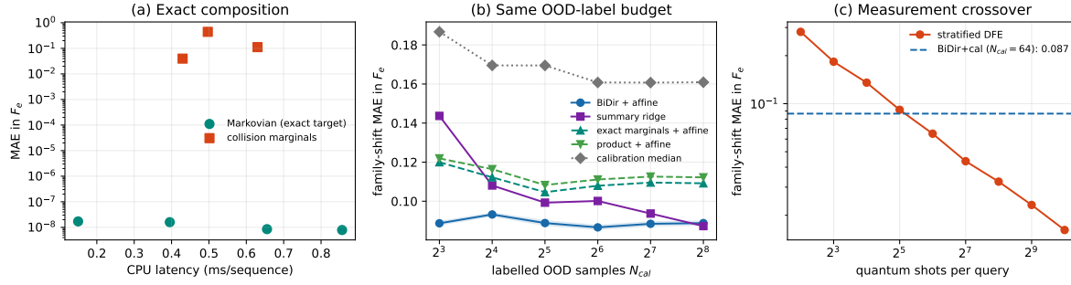
Figure 1. Negative controls and corrected cost-accuracy comparison. (a) Direct composition is numerically exact on Markovian full-Choi inputs at the studied d \leq 4 scale. Collision points use observable reset-bath marginals and retain an error from missing memory. (b) All OOD-calibrated methods receive identical labelled indices. (c) Stratified DFE reaches the calibrated neural error near 32 shots per query and gives a lower error at 64 shots.
