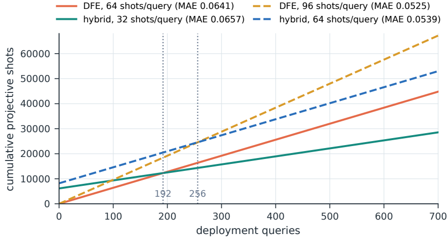
Figure 3. Full amortised measurement cost. The build cost includes 64 independent 64-shot target labels and 64 independent B -shot fusion pilots. The 32-shot hybrid and 64-shot Direct Fidelity Estimation have equal total cost after 192 queries at similar mean absolute error. The corresponding crossing for the 64-shot hybrid and 96-shot Direct Fidelity Estimation occurs after 256 queries.
