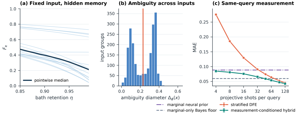
Figure 2. Diagnosing and repairing missing information. (a) Fixed marginal inputs can correspond to different fidelities as hidden bath retention varies. Curves show representative input groups. (b) The empirical ambiguity distribution yields a mean diameter of 0.229, a mean pointwise minimax floor of 0.115, and a uniform- \eta Bayes mean absolute error floor of 0.060. (c) A same-query Direct Fidelity Estimation pilot supplies information about the deployed process. In the highlighted regimes, the neural hybrid reaches the accuracy of this estimator using roughly one half to two thirds of its per-query shots. Error bars show run-to-run standard deviations.
