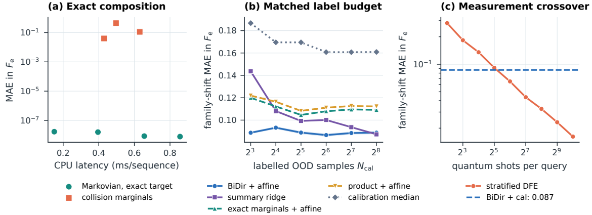
Figure 1. Negative controls and corrected cost-accuracy comparison. (a) Direct composition is numerically exact on Markovian full-Choi inputs at the studied d \leq 4 scale. Collision points use observable reset-bath marginals and retain an error from missing memory. (b) All out-of-distribution calibrated methods receive identical labelled indices. (c) Stratified Direct Fidelity Estimation reaches the calibrated neural error near 32 shots per query and gives a lower error at 64 shots.
