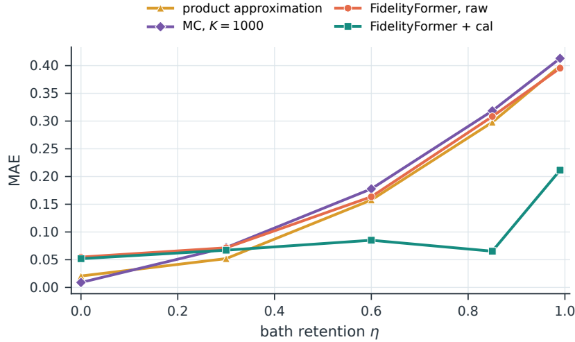
Figure 4. Bath-retention sweep for the decision rule. The retention coefficient \eta moves from reset-bath dynamics at \eta = 0 toward strong memory as \eta approaches one. Each point uses 1024 sequences. Neural curves average five seeds. Analytic and 1000-sample Monte Carlo curves use the same split.
