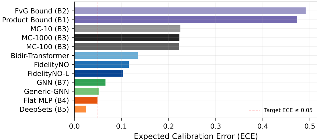
Calibration (ID Split)
