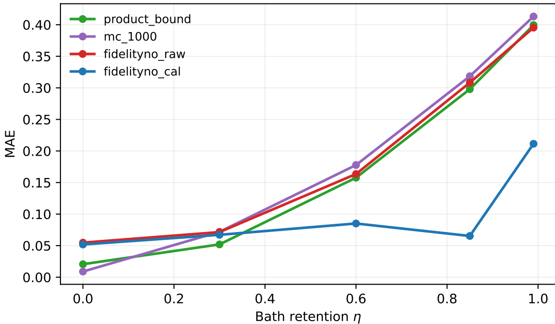
Collision-regime bath-retention sweep
