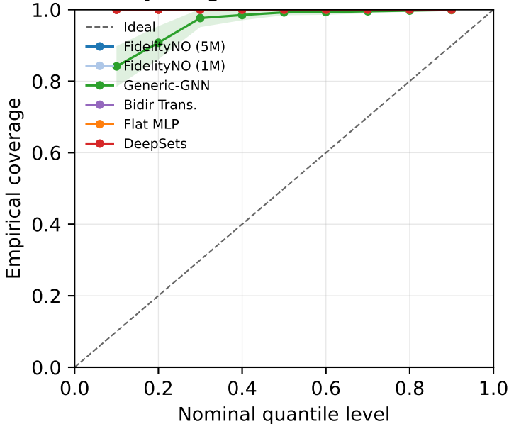
Reliability: length-OOD n = 48 (calibrated)
