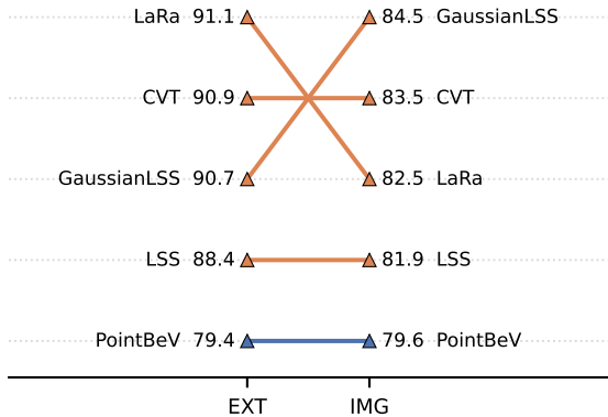
Segmentation
