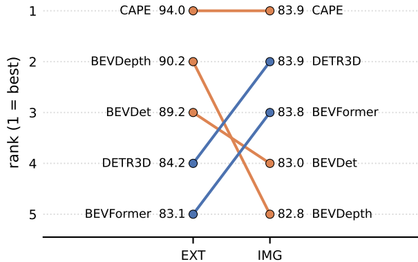
Detection
